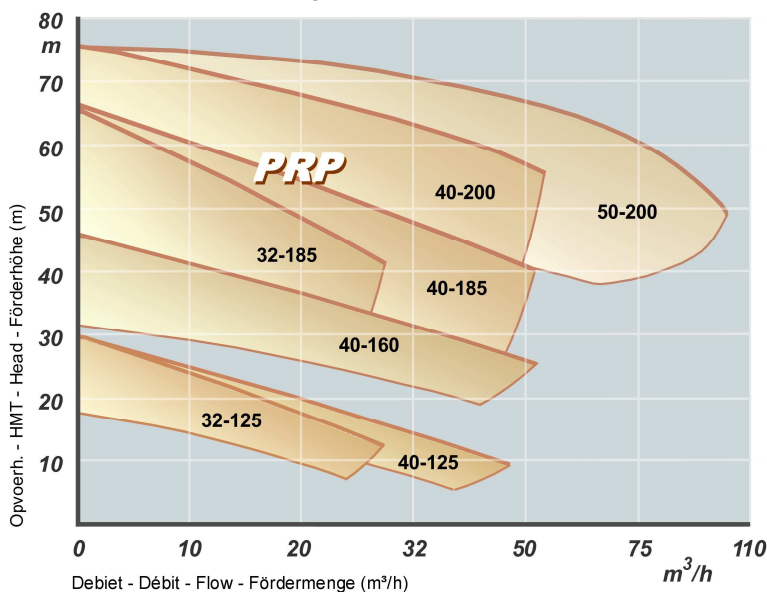
AIR HANDLING Pumps - Performance curves at 2900 RPM
